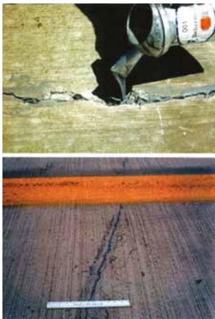
Fig. 3 – The transverse crack in the unjoined slab, repaired with epoxy, has remained closed ever since post-tensioning.
